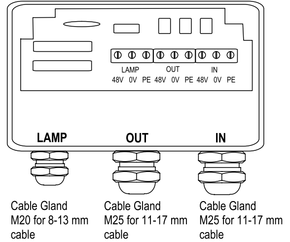
CEL-50-48-CST terminal box
