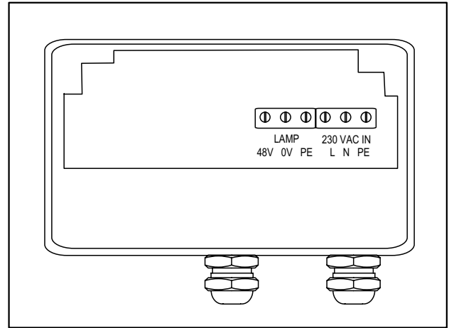
CEL-50-230-CST terminal box
