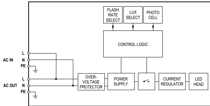
CEL-LI-32-115-PCFL block diagram
