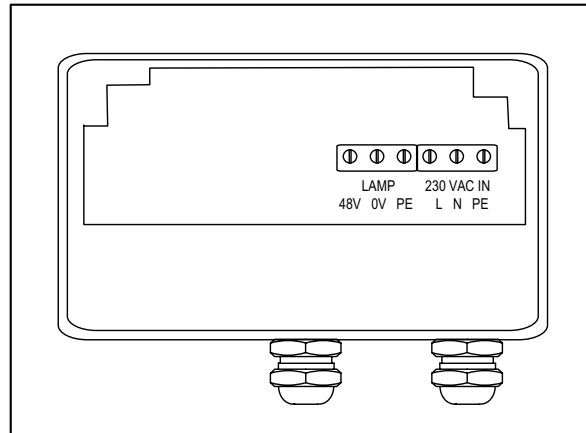
CEL-50-230-CST terminal box
